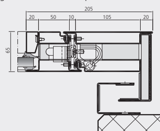
Sliding door EI30 with escape route function
